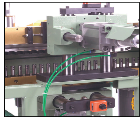
Rear View Of Independent Horizontal & Optional Independent Vertical Head
